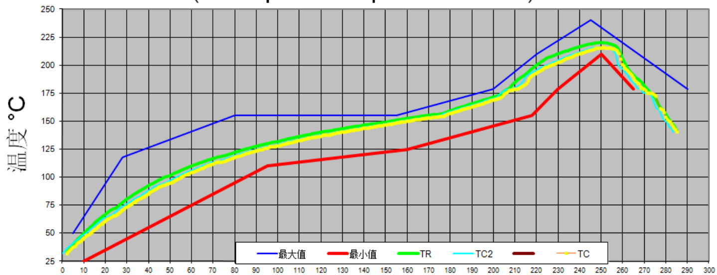
凹沉焊按温度曲线93cm/min (reflow profile at speed 93cm/min)
