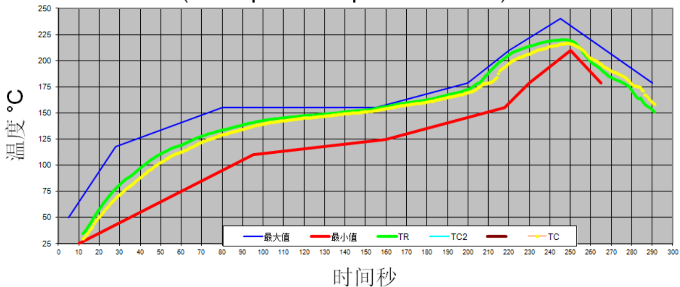
凹沉焊按温度曲线93cm/min (reflow profile at speed 93cm/min)
